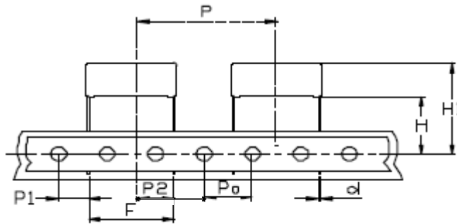
Fig 4 Pitch: 20.0/22.5/27.5 P 0 =12.7
