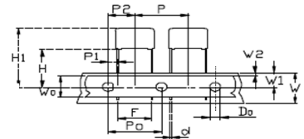
Pitch: /7.5 P 0 =12.7
