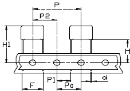
Fig 3 Pitch:10/12.5/15 P 0 =12.7
